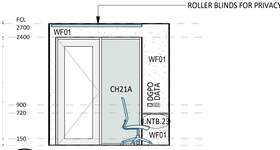
5 ELEVATION DETAIL 60-045 1 : 50
