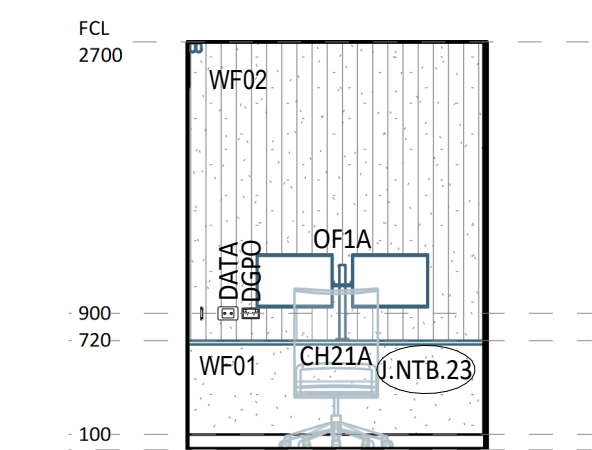
2 ELEVATION DETAIL 60-045 1 : 50
