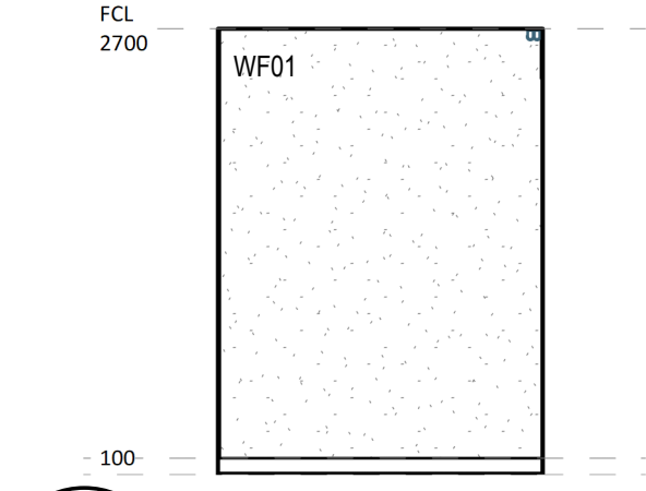
4 ELEVATION DETAIL 60-045 1 : 50
