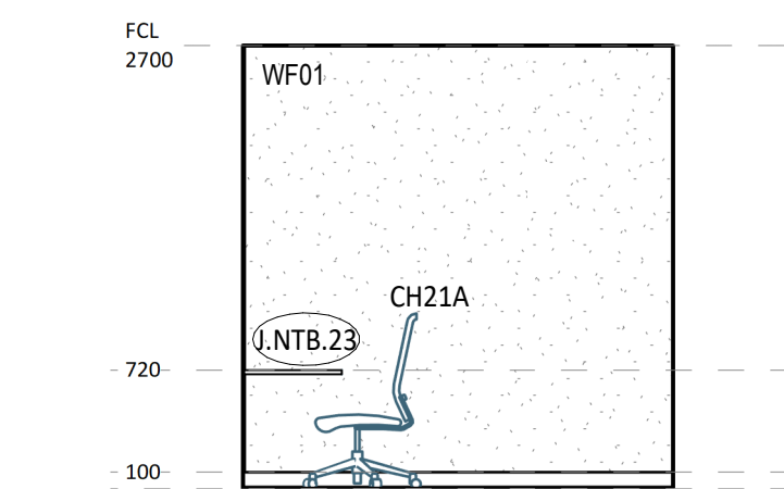
3 ELEVATION DETAIL 60-045 1 : 50
